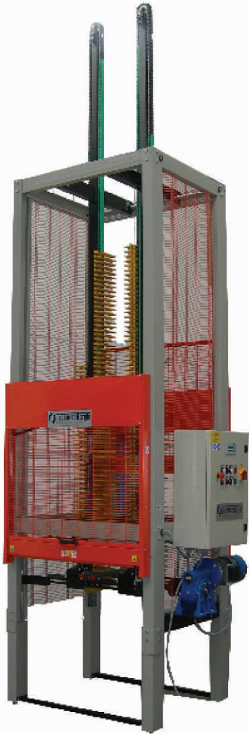
14) CMP – Compensatore verticale ad alette autoregolanti. CMP – Compensatore verticale ad alette. 14) CMP – Vertical compensator with self-adjustable tongues. CMP – Vertical slat compensator.
